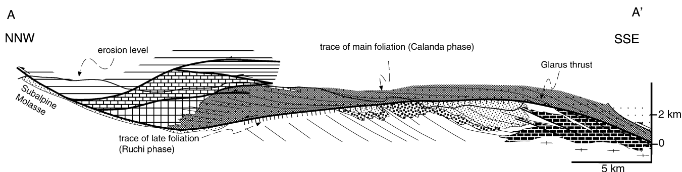
Fig. 3. Simplified cross section through Glarus Alps, modified from Schmid (1975) (see Fig. 2 for location and patterns for this section A–A').
