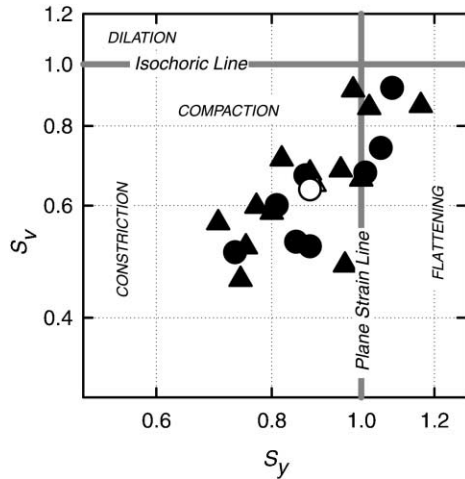
Fig. 7. Strain-type plot (Brandon, 1995) showing our absolute strain data: circles = lower plate samples, triangles = upper plate samples, closed symbols = individual determinations, and open symbols = tensor averages. The plot indicates a constrictional deformation ( S_Y < 1 ) with significant compactional volume strain ( S_V < 1 ).
