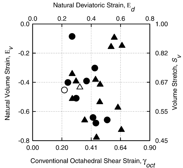
Fig. 8. The E_V - E_d diagram (Brandon, 1995) is used to compare the volumetric and deviatoric components of the strain. Our strain data show no correlation, which indicates that processes responsible for volume and deviatoric components of the deformation are, at least in part, decoupled: circles = lower-plate samples, triangles = upper-plate samples, closed symbols = individual determinations, and open symbols = tensor averages. E_V = \ln(S_V) and is a measure of volume strain. E_d is a measure of the average deviatoric strain, defined by E_d^2 = (1/3)[(E_x - E_y)^2 + (E_y - E_z)^2 + (E_x - E_z)^2] where E_x , E_y , and E_z are the natural logarithms of the principal stretches. E_V and E_d are linearly related to the principal strain rates for a coaxial deformation. Logarithmic axes are used to show equivalent values for the volume stretch S_V and the conventional octahedral shear strain \gamma_{oct} . See Brandon (1995) for further details.
