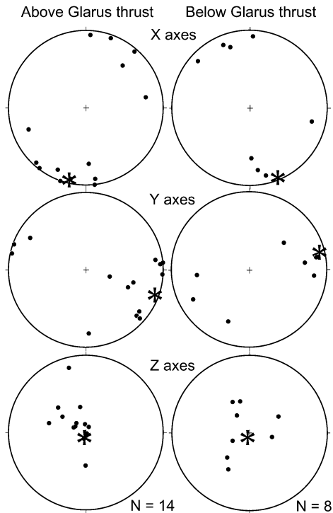
Fig. 5. Stereograms (lower-hemisphere, equal-area projection) of principal strain directions for samples above and below the Glarus Thrust (Table 1). The asterisks indicate principal directions for the tensor averages (Table 2).
