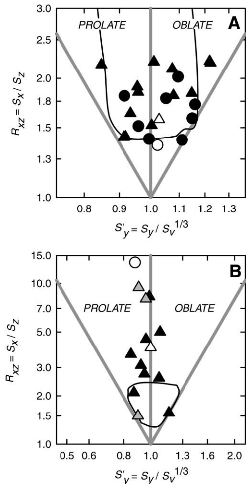
Fig. 6. Nadai plot showing strain symmetry and deviatoric strain magnitude (Brandon, 1995). S'_Y is the intermediate deviatoric stretch, equal to S_Y normalised to constant volume ( S'_Y = S_Y / S_V^{1/3} ). (a) Our measurements: circles = samples from below the Glarus Thrust, triangles = samples from above the thrust, closed symbols = individual determinations, and open symbols = tensor averages. The line outlines the lower end of the strain data distribution from Siddans (1979). (b) Previously published strain data from Siddans (1979) and Milnes and Pfiffner (1977): closed triangles (grey and black) = R_i/\phi measurements from Siddans (1979) for reduction spots in the Verrucano mudstones, located above the Glarus Thrust. The grey triangles mark results from localities near the Glarus Thrust. Open triangle = 'average' reported by Milnes and Pfiffner (1977) for the upper plate of the Glarus Thrust (probably determined from Verrucano reduction spots); open circle = 'average' reported by Milnes and Pfiffner (1977) for highly deformed rocks directly above the Glarus Thrust. The line outlines the distribution of our measurements.
