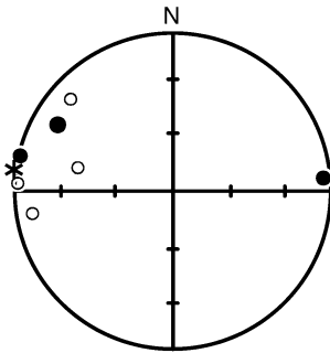
Fig. 9. Equal-area stereogram showing internal-rotation axes determined for samples from above the Glarus Thrust (Table 1). Points are right-handed rotation vectors, with closed and open symbols indicating lower and upper hemisphere directions, respectively. Six out of the seven measurements indicate a consistent top-north shear sense. The asterisk shows the mean direction for the internal-rotation axes (Table 2), which also shows a top-north shear sense.
