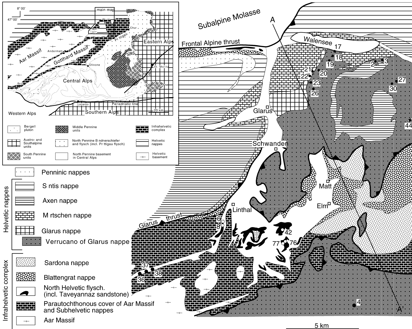
Fig. 2. Structure map of the Glarus Alps, adapted from Lihou (1996). Numbers show localities for samples reported in Table 1. The line A–A' locates the cross-section shown in Fig. 3. The inset map shows the major tectonic zones of the Central Alps.
